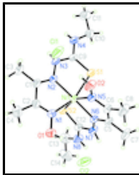
Fig. 1. The molecular structure of the title compound, with 50% probability displacement ellipsoids and the atom-numbering scheme.
